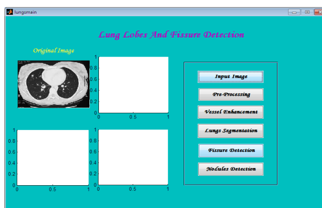
Fig 4.1 Input screen
